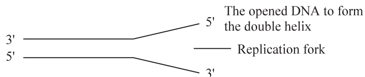
Fig. 23.7a Replication fork
